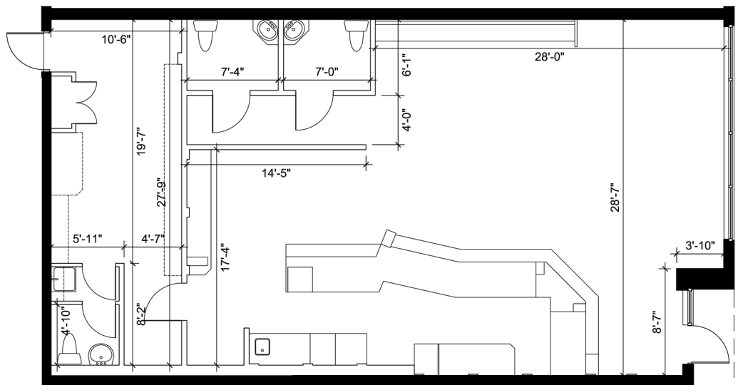
KEYPLAN
